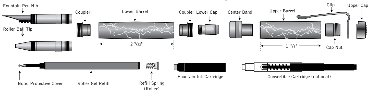
DIAGRAM C / Pen assembly
